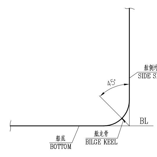
舷龙骨安装位置示意图 BILGE KEEL MOUNTED POSITION SKETCH MAP
